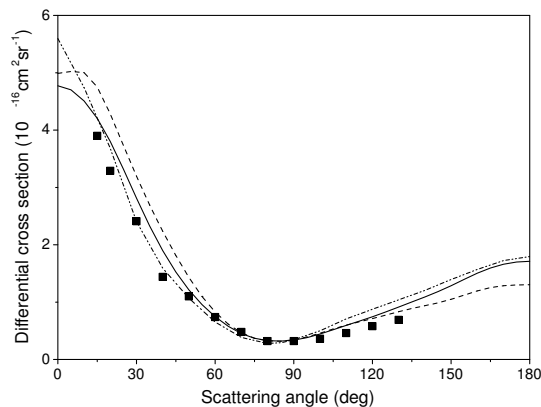
FIG. 4: DCS for elastic electron scattering CO at energy of 15eV: —, present SDCI results; — — —, present HF results; — · —, theoretical results of Rolles et al. [33] and \blacksquare , experimental data of Tanaka et al. [32].
