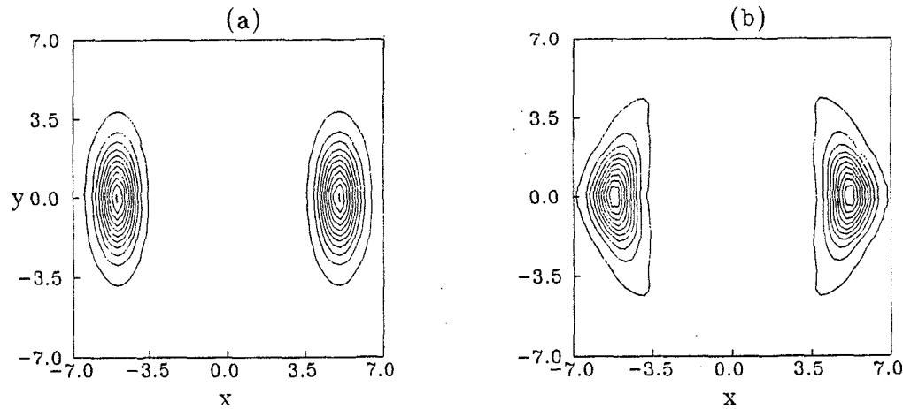
Figure 5: Q -function contours for an initial field prepared in a superposition of squeezed coherent states with r = 1 and \alpha = 5 , at: a) t = 0 ; b) t = T_r .
