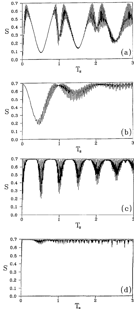
Figura 4: Field entropy for an initial field prepared in: a) a squeezed coherent state with r = 1 ; b) a squeezed coherent state with r = -1 ; c) a superposition of squeezed coherent states with r = 1 ; d) a superposition of squeezed coherent states with r = -1 . In all cases a = 5
