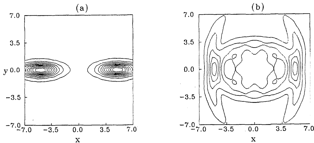
Figure 6: Q -function contours for an initial field prepared in a superposition of squeezed coherent states with r = -1 and \alpha = 5 , at: a) t = 0 ; b) t = T_r .
