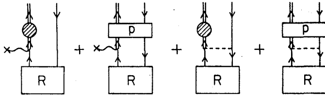
Fig.2 - Virtual background space component emanating from the resonance-hole component. The first two contributions involve one-body coupling between resonance-hole and background spaces, the last two involve two-body coupling. The second and fourth contributions contain channel coupling effects.
