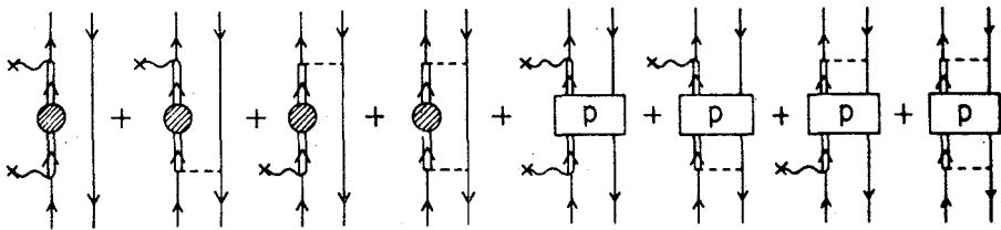
Fig.3 - Contributions to the effective resonance-hole interaction, second term on the right-hand side of eq.(3.8). The middle part of each contribution involves one of the possibilities of propagation in p-space and coupling to the resonance-hole space goes either through one- or two-body processes. Symbols are as in figs. 1 and 2.
