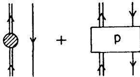
Fig.1 - Particle-hole scattering within the background subspace. The first contribution involves elastic scattering of the particle in the presence of a spectator hole, and the second indicates channel coupling processes.
